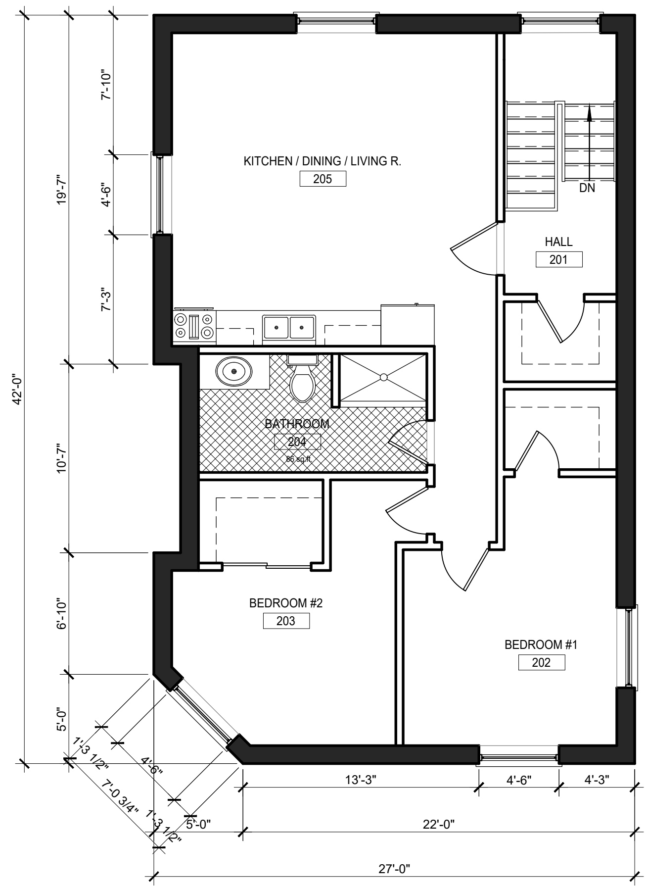
1 2ND FLOOR PLAN A-103 3/16"=1'-0"
