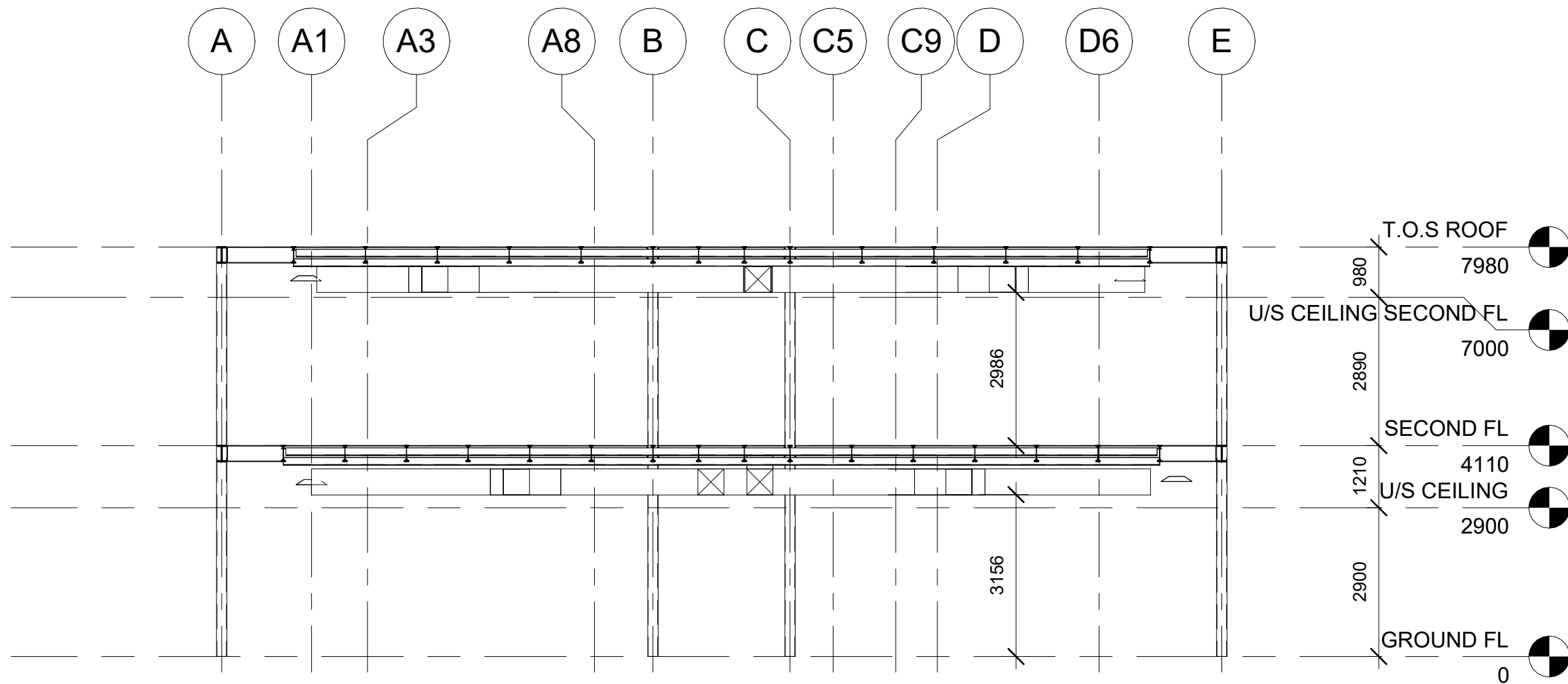
1 BUILDING SECTION 1 : 100
